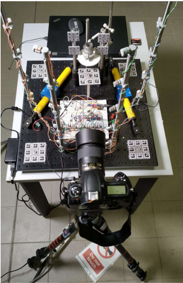
Prototype system (left) developed by the 3DOM unit that fuses photogrammetry and photometric stereo techniques for the 3D inspection of industrial components (right).
