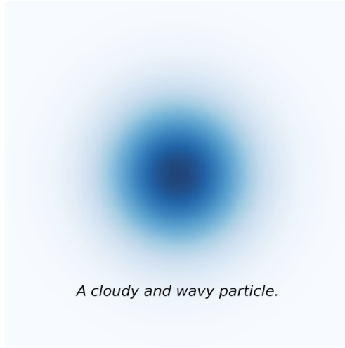
Quantum particle
