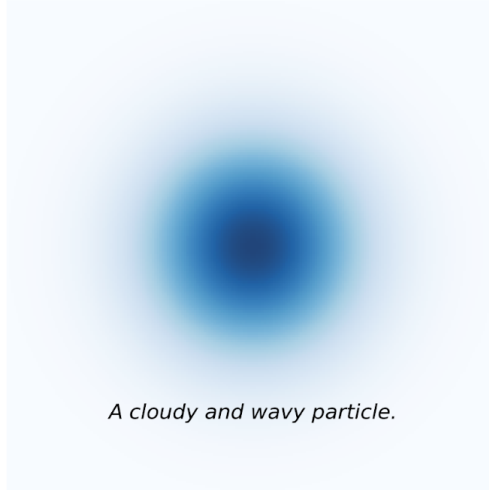
Quantum particle
